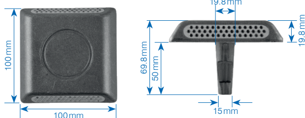
Plots routiers AluFIX
