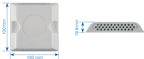
Plots routiers AluFIX
